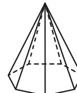
heptagonal pyramid
