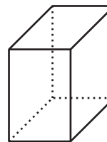
rectangular prism
