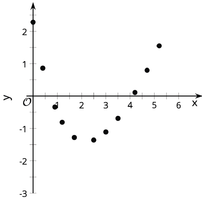
Best Residuals
