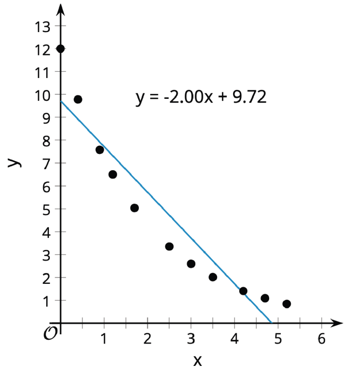
Best Residuals
