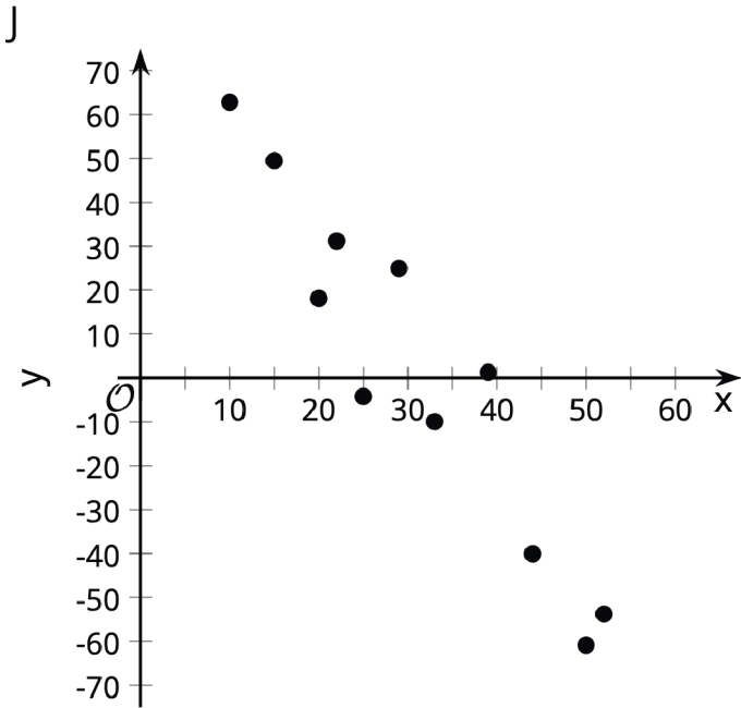
Best Residuals
