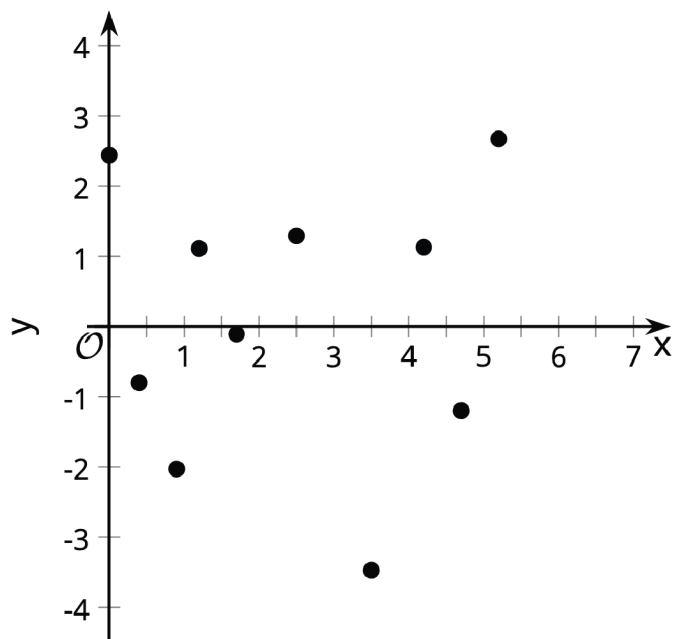
Best Residuals
