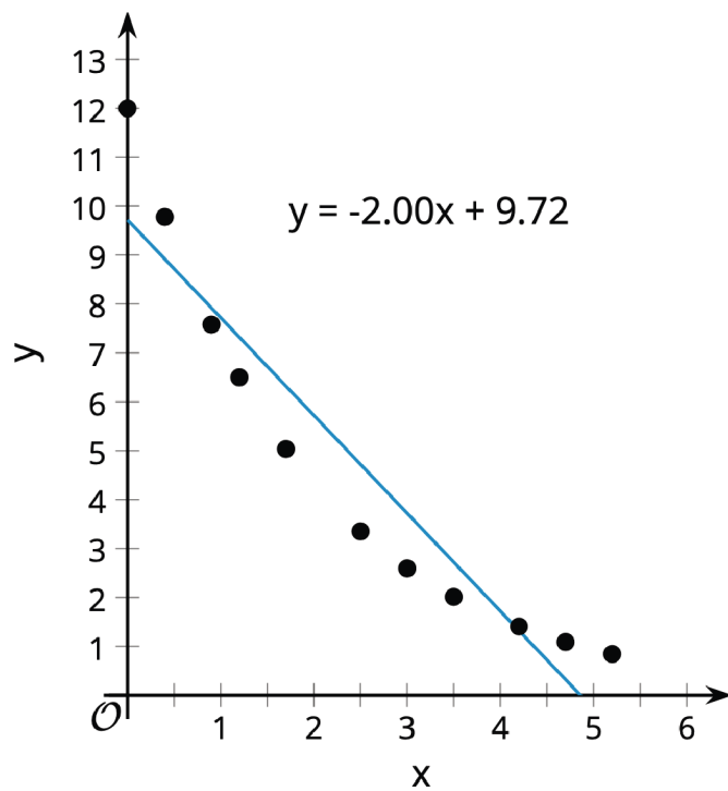
Best Residuals
