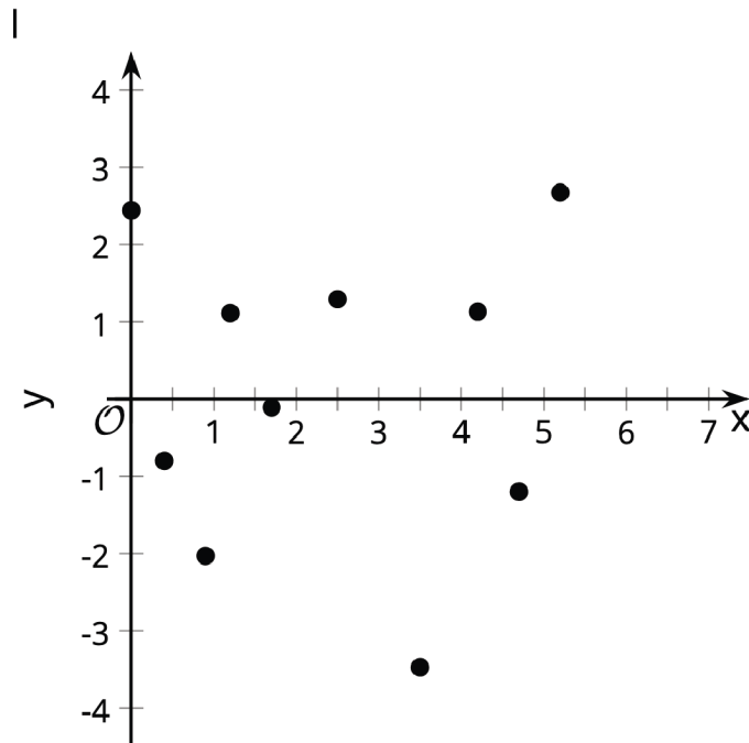
Best Residuals
